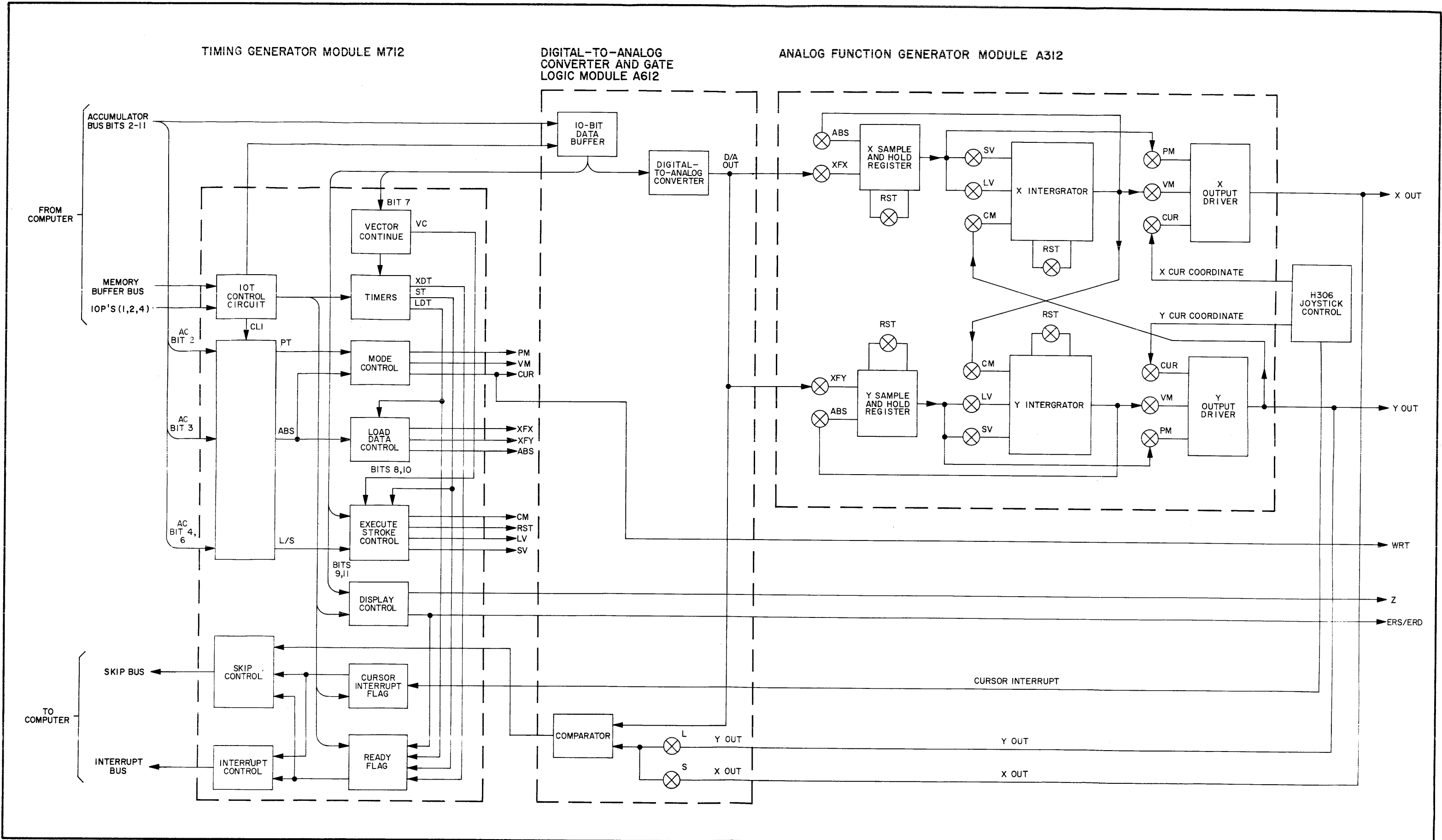
Figure 4-6. KV Controller Functional Block Diagram
